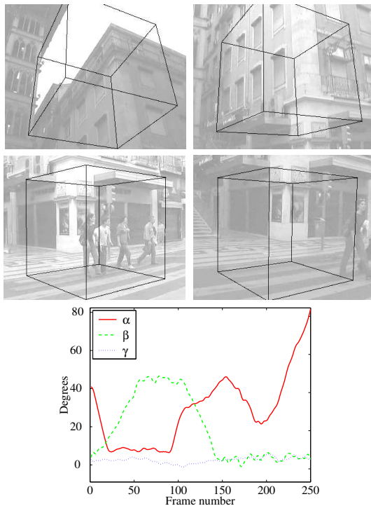
Fig. 7. Top: frames 110, 130, 150, and 170 of a third video sequence. Bottom: camera angle estimates.
