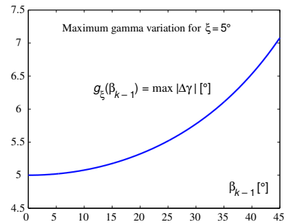
Fig. 4. Maximum variation for the twist angle as function of the initial elevation angle, using a SR(5^\circ) model.
