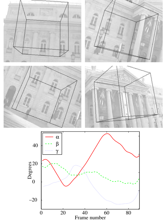
Fig. 6. Top: frames 20, 30, 40, and 50 of another video sequence. Bottom: camera angle estimates.
