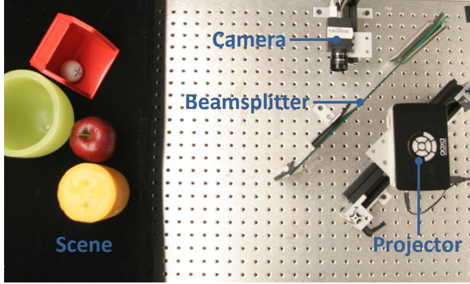
Figure 2.5: Experimental Setup: Our experiments were performed using a camera and projector colocated with a plate beam splitter. We also have a portable version of the setup.
