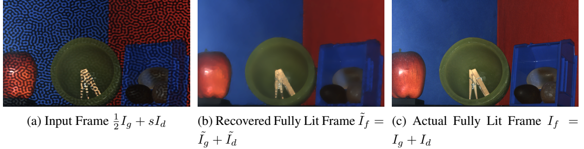
Figure 2.3: Recovering a Fully Lit Image: An image captured under a known high frequency illumination pattern (a) is relit to form an estimate (b) of how the scene would have appeared under uniform lighting. For reference, the actual appearance of the scene under uniform lighting is shown in (c). The relit estimate (b) captures the structure of the scene fairly well but smooths over some of the finer detail that is visible in (c) and the regularization introduces some artefacts (notice the pegs placed inside the green bowl). Relit images are used to perform image alignment on the original images
