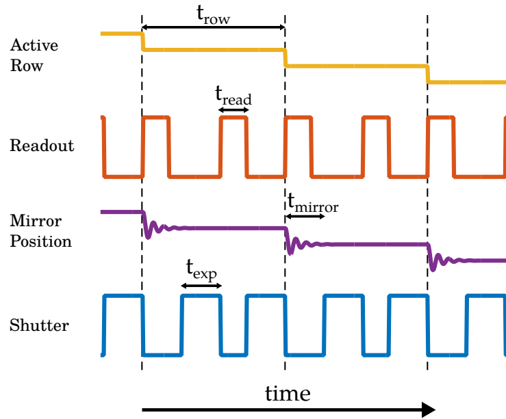
Figure 5.5: Timing diagrams for camera exposure, readout and mirror position for a particular sequencing of the rows. First, the scanning mirror is moved to the new active row and takes t_{\text{mirror}} to settle in the position. When the previous row readout is complete (which takes t_{\text{read}} ) and the the mirror is in position, the camera is triggered. Each exposure lasts for t_{\text{exp}} and at the end of each exposure the row is read out.
