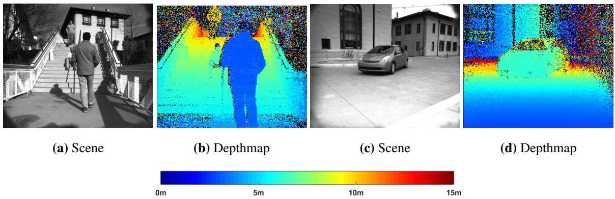
Figure 5.8: Depthmaps from our epipolar ToF camera outdoors on a sunny day. The camera modulation frequency is 10 MHz and so the maximum ambiguity-free range is 15 m. The resulting wrap around in depth values is noticeable in the wall behind the car in (d) which is more than 15 m away.
