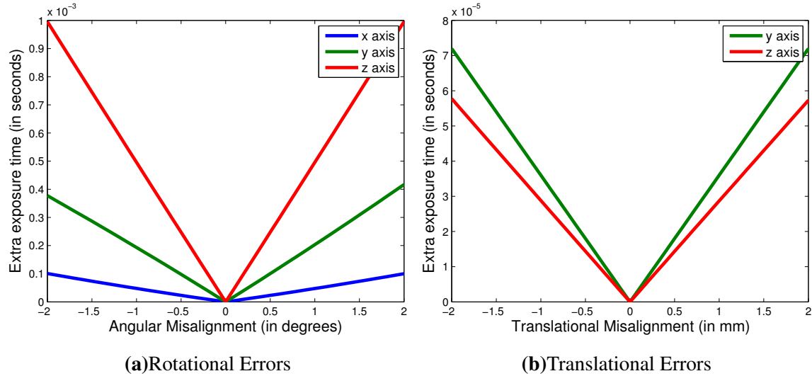
Figure 4.13: Alignment Analysis: The Episcan3D sensor needs its projector and camera to be physically aligned in a stereo configuration. As the projector goes out of alignment with one of the cameras, the camera exposure needs to be increased for the epipolar light to be captured by the rolling shutter masks. When correctly aligned, our current prototype uses an exposure time of 100\mu s . Increasing the exposure time by another 100\mu s to provide slack for misalignment would double the amount of ambient light reaching the sensor. In (a) the slack exposure required for rotational misalignments along the various axes is plotted. The system is relatively less sensitive to rotations about the projector’s x axis because these can be corrected for (to a point) in software by adjusting the trigger offset. In (b) we plot slack exposure required against translational misalignment. Misalignment along the x axis alters the baseline but does not affect rectification.
