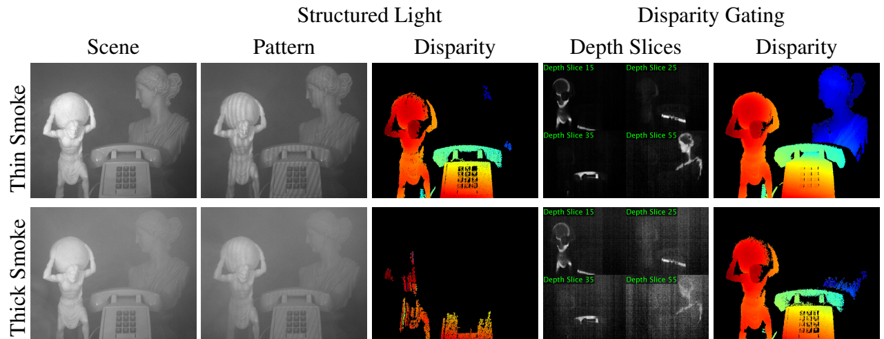
Figure 4.11: Disparity gating in participating media. We compare structured light with regular imaging to disparity gating. Disparity Gating is able to reconstruct objects at a further distance through the smoke than regular structured light. For structured light, we use 20 patterns and average 3 16.67ms exposures for each pattern. For disparity gating we divide the range of disparities in the scene into 60 slices and capture each slice with a 16.67ms exposure.
