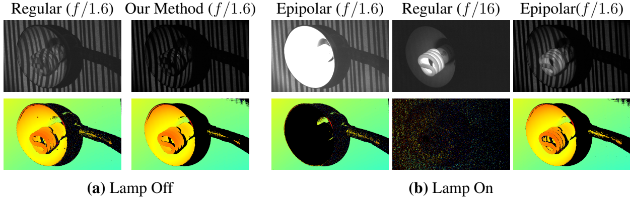
Figure 4.6: Imaging and scanning a 1600 lumen lamp with a 15 lumen projector: When the lamp is off (a), the pattern projected by the projector is visible with both regular imaging and with epipolar-only imaging. By projecting a series of structured light patterns the lamp can be reconstructed. When the bulb is turned on (b), regular imaging breaks down. With a large aperture ( f/1.6 ), the image is saturated, with a small aperture ( f/16 ) the projected pattern is not visible to the camera on the bulb or the shade. In epipolar-only imaging mode, the Episcan3D sensor exposes camera pixels only while they can receive light from the projector and as a result, most of the light from the bulb is blocked, the pattern is clearly visible even on the bulb and the fixture can be reconstructed even though it is on.
