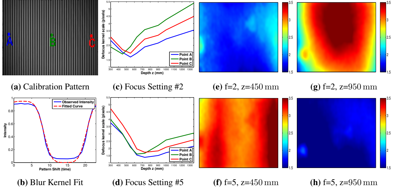
Figure 3.1: Characterizing Projector Defocus: (a) - image of one of the square wave patterns for estimating projector blur. (b) is the temporal intensity profile at point B and the Gaussian smoothed square wave fit. (c) and (d) - the blur kernel scale \sigma for the projector pixels A,B and C for two different focus settings as the scene depth is varied. (e) to (h) - maps of blur scale \sigma across the projector image for different combinations of focus setting and scene point depth. The value of \sigma clearly varies across the image, especially when the projector is out of focus.
