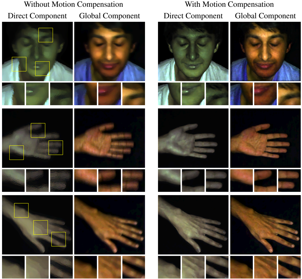
Figure 2.8: Direct-Global Separation on Skin: On the left are the global and direct components estimated without any motion compensation for a face changing expression and articulating hands. Many details get blurred away like the hair, and the lines on the palm. Other motion artifacts are clearly visible on the fingers. The two columns on the right show the component estimates on the same frames using our motion compensation method. With motion compensation, many of the artifacts are corrected and a lot more of the original scene detail is recovered. In the face example, some of the subsurface scattered light leaks into the direct images giving them a slightly greenish tinge. This happens because the subject is somewhat further away and the projected patterns at the subject are not high enough frequency to completely resolve the subsurface scattered light. A similar effect was observed in [70].
