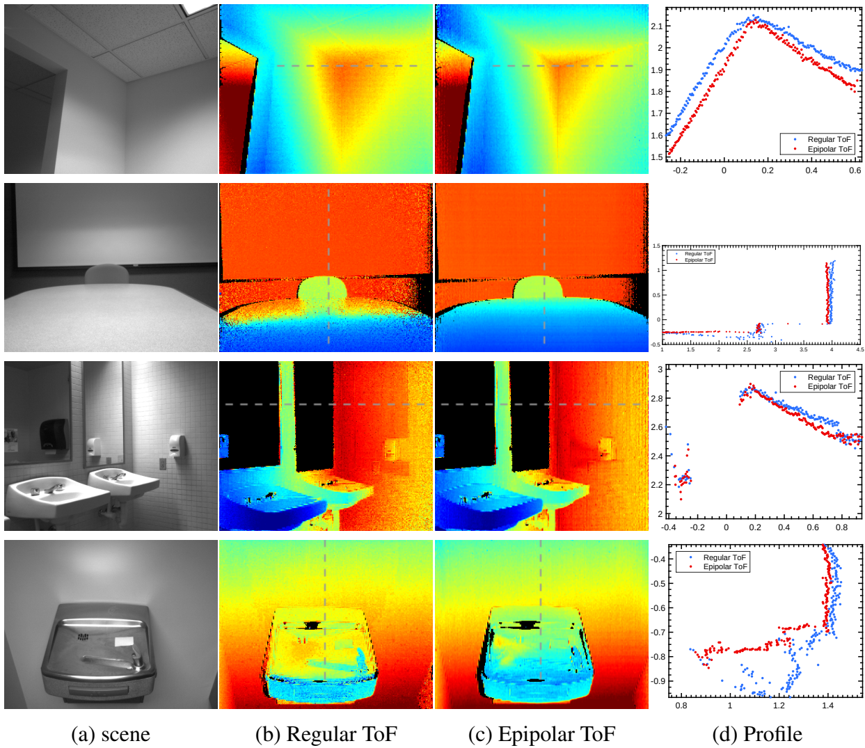
Figure 5.10: Comparing depth maps with epipolar and regular ToF imaging in the presence of global light transport: diffuse interreflections at the corner, glossy interreflection from projection screen onto a shiny conference table, reflections from the mirrors in the restroom and in between the wall and the shiny water fountain. Epipolar ToF eliminates most of the global light transport resulting in depth maps that are significantly more accurate than regular ToF. All profile curves are in meters.
