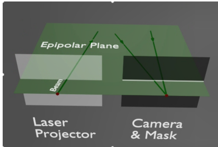
Figure 4.1: Energy-Efficient Epipolar Probing. A raster-scanning projector is combined with a camera sensor with maskable pixels. The projector and camera are placed in a rectified stereo configuration so that by epipolar geometry, each projector scanline corresponds to a row of pixels in the camera. To perform epipolar-only probing the camera mask is configured so that at any point of time, only the row of pixels corresponding to the active projector scanline is exposed. To implement non-epipolar probing, the camera masks are inverted - only the row corresponding to the active scanline is masked, all other pixels are exposed.
