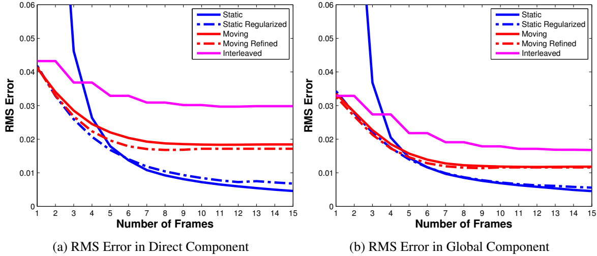
Figure 2.6: Comparison of Separation Techniques: The RMS errors in the direct (a) and global (b) components for different separation techniques as the number of frames used is varied. The blue ‘static’ curves are from direct-global separation on stationary scenes and represent the best possible performance a method could achieve for a given number of frames. The red ‘moving’ curves are from using our motion compensation algorithm on moving scenes. When the number of frames is small, the motion compensation method performs just as well on the moving sequences as normal separation on an equal number of static frames. When the window size increases, frames far away from the window center are discarded because alignment fails and so performance of the motion compensated algorithm levels off.
