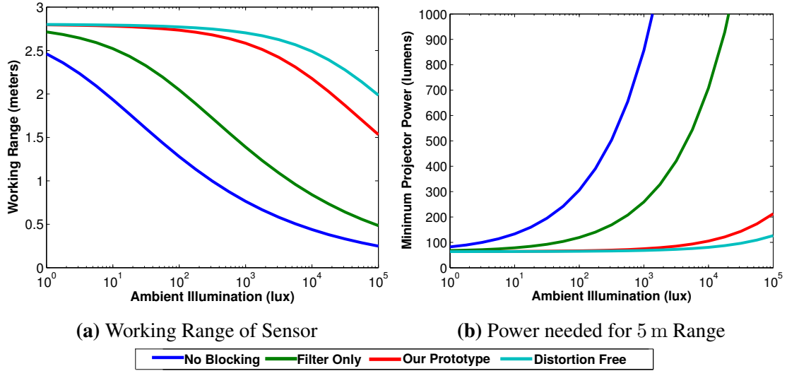
Figure 4.12: Range analysis. (a) Maximum working range of a system with the same projector light output and cameras as our sensor as a function of ambient light level for different ambient blocking schemes. (b) The projector power required to attain a 5 m range. By effectively blocking a large fraction of the ambient light, epipolar-only imaging with a laser projector is able to provide energy-efficient operation even under bright ambient illumination conditions. Code listings for this analysis appear in the appendix.
