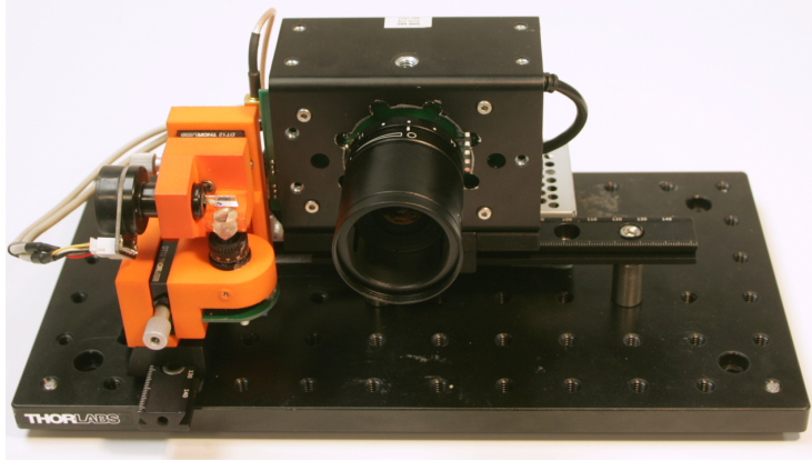
Figure 5.4: Our Epipolar ToF prototype uses a custom built steerable light sheet projector (orange assembly) and a DME660 camera with fast ROI control to capture arbitrary rows of pixels.
