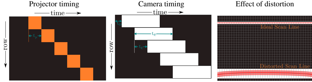
Figure 4.3: Electronic masking with a rolling shutter: At each timestep (of duration t_p ), the projector illuminates a single scanline (top left). The camera uses its rolling shutter to selectively mask pixels (top right). The masks are defined by three controllable parameters, the exposure time t_e , the time it takes the rolling shutter to read a row of pixels t_c and the offset between the projector sync output and the camera trigger input t_o . Ideally, a single projector scanline corresponds to a single camera row. In practice, because of distortion and jitter, each scanline corresponds to a band of camera pixels.
