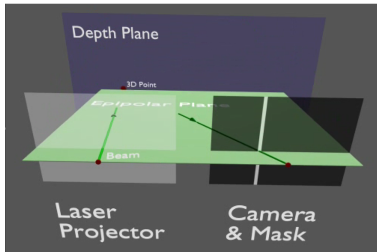
Figure 4.10: Geometric Arrangement for Disparity Gating. By rotating both the projector and camera in figure 4.1 by 90^\circ around their optical axes, the projector scanlines and camera rows become perpendicular to the projector-camera baseline. If the projector and camera are synchronized so that there is a fixed offset between the active projector scanline and the exposed camera row, the image captured contains only light paths corresponding to a single disparity value - a single depth plane in the scene.
