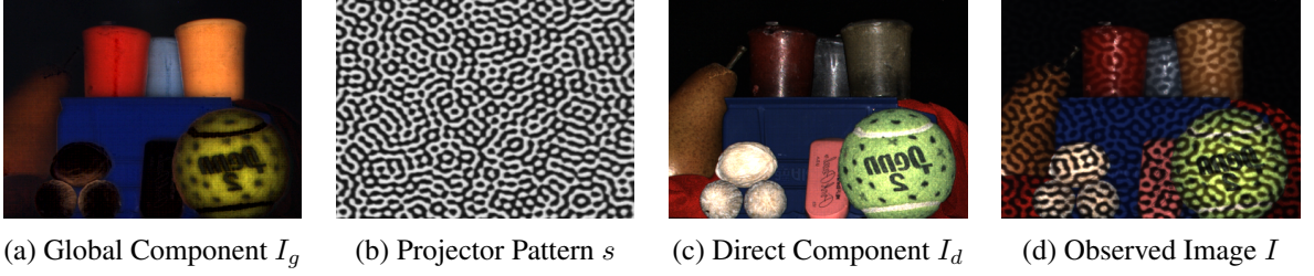
Figure 2.2: Image Formation Model: The observed image I is modeled as a linear combination of the global component ( I_g ) and a projector pattern ( s ) modulated version of the direct component ( I_d ). I = \frac{1}{2}I_g + sI_d . The specularities on the candles appear in the direct image and most of the color is due to subsurface scattering in the wax and appears in the global image.
