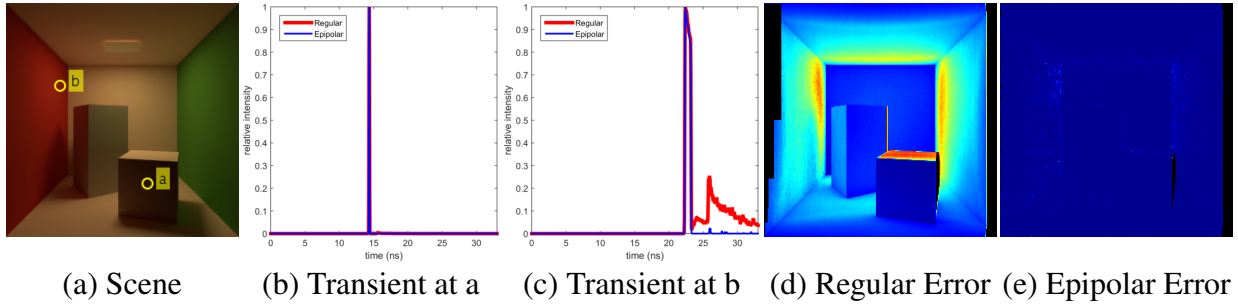
Figure 5.2: Simulation showing the effects of global illumination on continuous wave time-of-flight with regular and epipolar imaging. (a) a Cornell box scene - for scale, the back wall is roughly 3.7 m from the camera. (b) at point a - on the cube in the foreground, there is little global illumination so the transient responses under both regular and epipolar imaging are close to impulse responses. (c) at point b - near the corner on the red wall, there is a strong inter-reflection which shows up as a long tail in the transient response under regular imaging which is largely suppressed in epipolar mode. (d) shows the difference between the groundtruth depth and depth estimated using regular imaging CW ToF (modulation frequency 30 MHz) as a heatmap (scaled between 0 cm and 50 cm), there are large errors due to interreflections. (e) the same error visualization for epipolar imaging, almost all the errors are suppressed.
