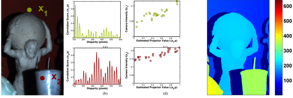
Figure 3.4: Establishing Correspondences: Part of a scene (left) and the computed disparity map (right). Graph (a) shows the correlation score for point x_1 as a function of disparity to the projector. The disparity that leads to the best match is 115. There are many peaks in the correlation score graph, but modeling of illumination blur causes the peaks to decay as we move away from the correct disparity value. Graph (c) shows the intensity observed by the camera against the simulated projector illumination value for the best disparity. Graph (b) and (d) are the same trends for point x_2 . Because of strong sub-surface scattering at x_2 , the global illumination component is large and the direct component is relatively small. This can be seen in (d).
