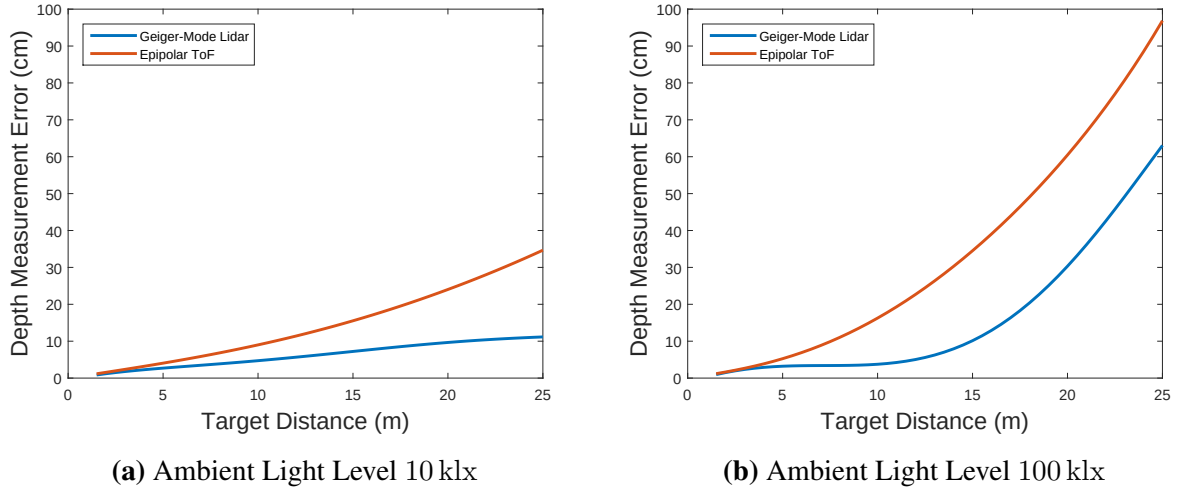
Figure 6.2: Simulated Comparisons of Epipolar CW-ToF to Geiger-Mode Lidar. For parameters of the simulated Epipolar CW-ToF camera see table 5.2. The Geiger-Mode lidar light source emits 100 pulses per depth reading, with a pulse length of 5 ns and per-pulse energy of 288 \mu J. This makes the energy emitted per depth frame equal for both sensing modalities. Field of view, operating wavelength, sensor size and other parameters were also kept equal in both simulated systems. For the simulated Geiger-Mode sensor, the photon detection probability is 0.1, the detection jitter is 100 ps and the lens aperture is set to f/4 . (a) compares the two systems under the equivalent of cloudy conditions, (b) compares the two systems under bright sunlight.
