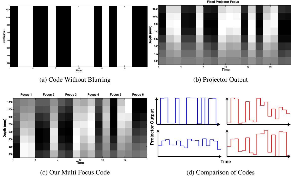
Figure 3.3: Effect of Defocus on Codes: When illumination defocus is not modeled, the temporal code associated with a projector pixel (a horizontal cross section of (a)) is independent of depth. However, as (b) shows, outside a narrow working range, the actual appearance of the code is depth dependent. In (c), we use 6 focus settings and 3 patterns per focus. Using multiple focus settings allows us to expand the systems working volume. Also, we model illumination defocus so blurred codes do not cause errors. When regular codes are in focus, they work well (upper blue graph in (d) ), however for scene points that are out of focus, contrast is very poor (lower blue graph in (d) ). On the other hand, our multiple focus codes always have parts that are well focused and thus have high contrast (red graphs in (d)).
