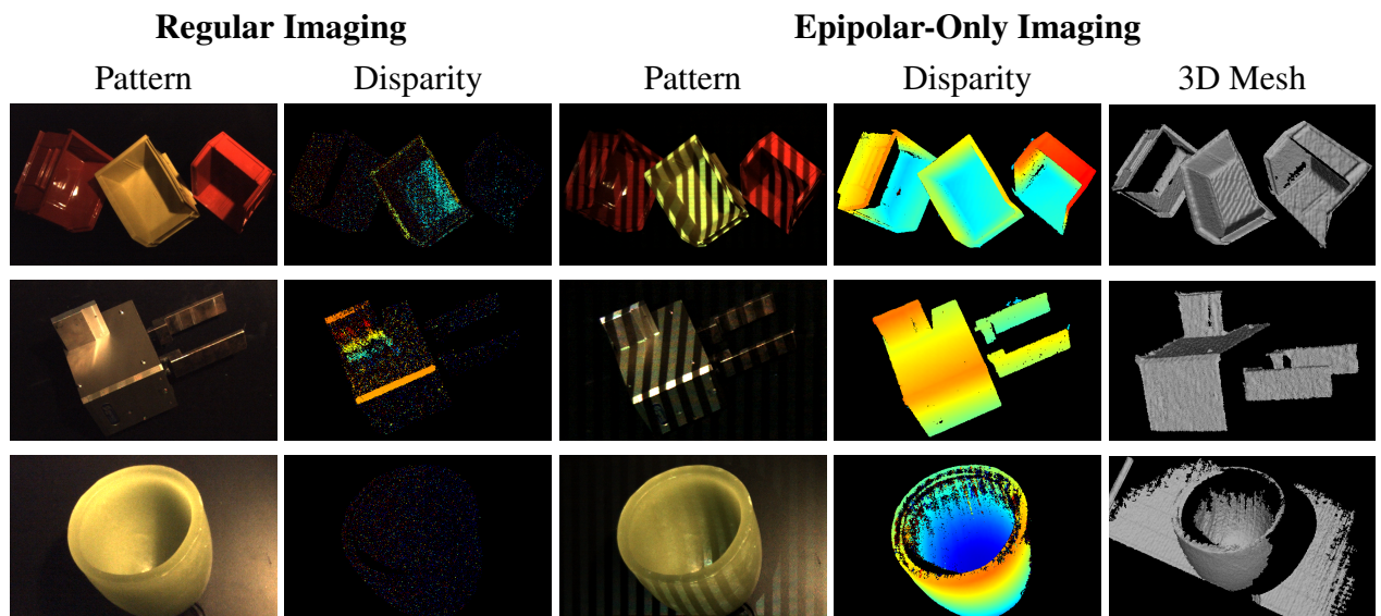
Figure 4.8: Scanning Objects Under Bright Ambient Lighting: These objects are being scanned using structured light while simultaneously illuminated by a bright indoor spotlight (ambient light level is approximately 10 klx). In these examples, there is no wavelength filter attached to the camera. With regular imaging the patterns can not be detected by the camera and the reconstructions are poor. With epipolar-only imaging, the plastic bins and gripper are reconstructed well. The wax bowl reflects very little light directly, most light scatters below the surface so it is particularly difficult to scan under bright ambient light.
