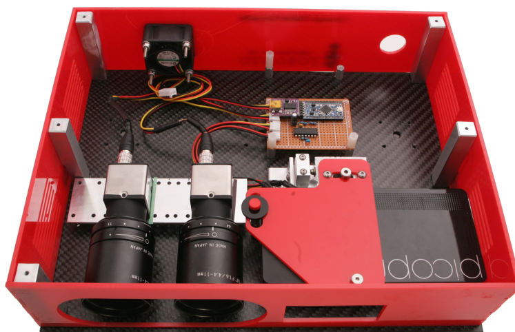
Figure 4.2: Episcan3D Hardware Implementation: The Episcan3D sensor consists of a low power raster scanning laser projector, a pair of CMOS rolling shutter cameras and a microcontroller for synchronization. There is no dedicated hardware for masking on the camera side as the camera rolling shutters are used to perform masking.
