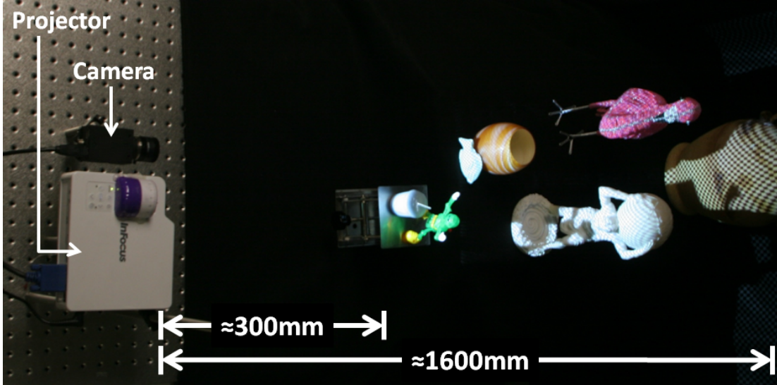
Figure 3.6: Experimental Setup: With a small, 500 lumen DLP projector that has limited depth-of-field and a small number of images, we are able to scan scenes over a large working volume to recover accurate depth maps and perform illumination separation.
