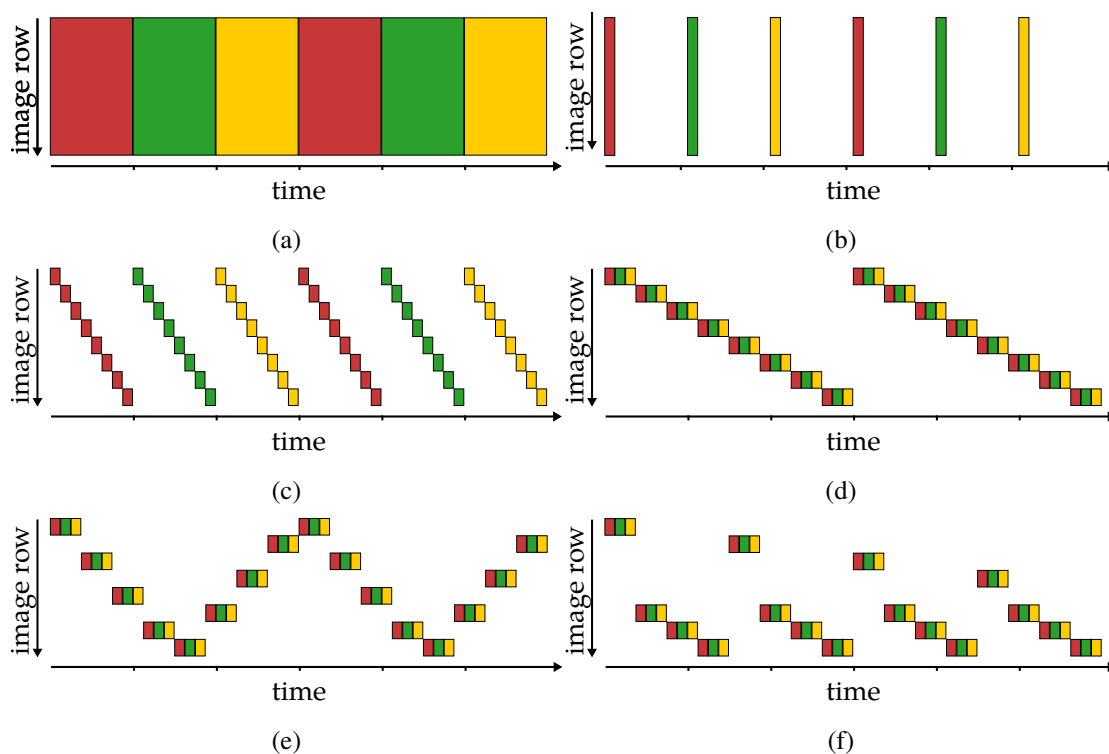
Figure 5.3: Epipolar plane sampling schemes and row exposures in ToF imaging. (a) In conventional CW-ToF all epipolar planes are illuminated simultaneously and all camera rows are exposed at the same time. This requires long exposures and leads to severe artifacts due to motion, ambient light, global light transport and interference between devices. (b) Sending a very brief, high-intensity pulse of light for CW-ToF confers resistance to ambient light but is still prone to artifacts due to global light transport and motion. (c) Ordering the epipolar ToF planes similarly to a rolling-shutter camera confers robustness to ambient light, global illumination and motion blur. Sensitivity to motion remains, however, because of the significant delay between the phase measurements acquired for each row. (d) Interleaving those measurements plane by plane minimizes such artifacts. (e) Scanning the entire field of view twice within the same total exposure time yields higher temporal sampling of the scene and makes consistent merging of individual depth map rows easier. (f) For certain applications, scanning different portions of the field of view with different temporal sampling rates can be beneficial.
