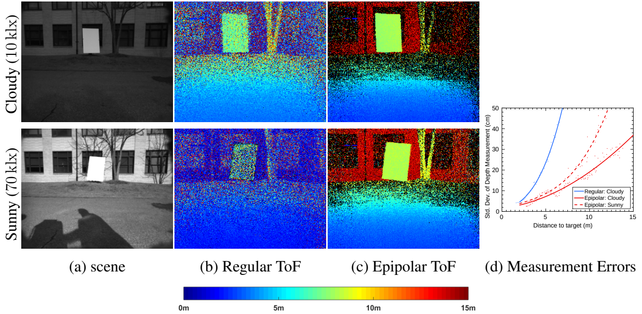
Figure 5.7: We placed a white planar target at a range of distances from the sensor in both cloudy weather and bright sunshine. Even under cloudy conditions, epipolar ToF imaging produced far less noisy depth measurements than regular ToF. Under bright sunlight, regular ToF failed completely whereas epipolar ToF still provided useful depth returns. The camera modulation frequency was set to 10 MHz. (d) shows standard deviation in depth estimates versus distance to target (slower rising curves are better). Our prototype has depth error of around 3% at 10 m in bright sunlight.
