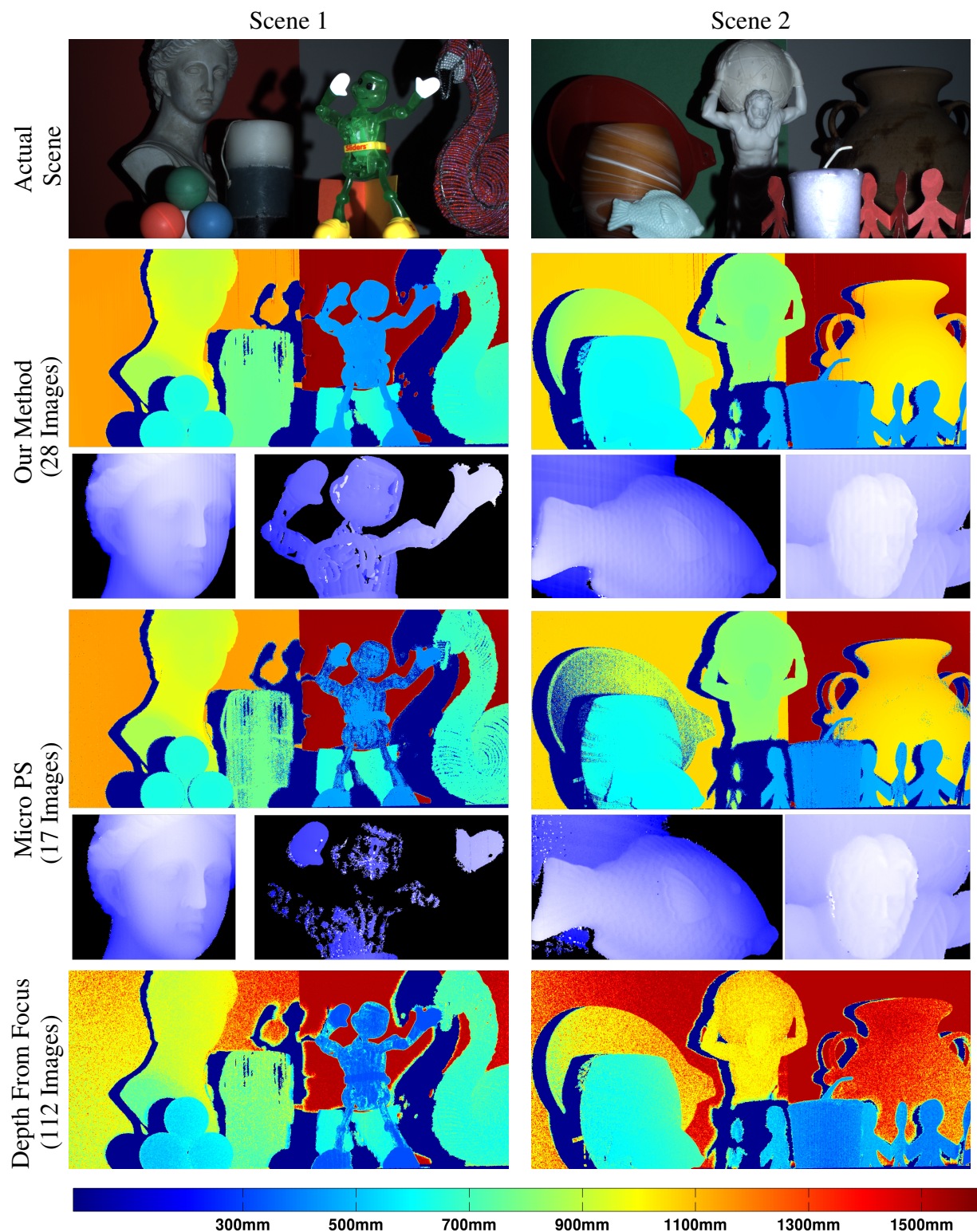
Figure 3.7: Our algorithm recovers depth maps for scenes containing challenging objects over an extended working volume with relatively few images. Insets show (rescaled) depth maps for small parts of the scene. Fine details like the scales on the soap fish are successfully resolved.
