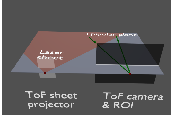
Figure 5.1: Epipolar time of flight. A projector that generates a steerable sheet of modulated laser light is combined with a ToF sensor whose rows can be exposed one at a time. The projector and camera are placed in a rectified stereo configuration so that the light sheet always lies on an epipolar plane between the projector and the camera. At any given instant, only the row of camera pixels on the epipolar plane is exposed to light..
