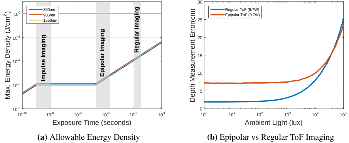
Figure 6.1: (a) In the near-infrared band, the permissible energy density of a light source is a function of exposure time. As a result, for a given eye safety requirement, regular imaging with a non-redistributive light source can use much higher power than epipolar imaging with a line striping source. (b) compares the accuracy of two CW ToF systems with the safe eye safety characteristics - one using regular imaging and another using epipolar. The target distance is fixed at 10 m and ambient light levels are varied. Despite using roughly 14 time less energy, epipolar imaging would still be more accurate than regular imaging in bright sunlight. For short-wave infrared, the maximum allowable energy density is much higher and doesn't depend on exposure time, but SWIR sensors are expensive and difficult to fabricate.
