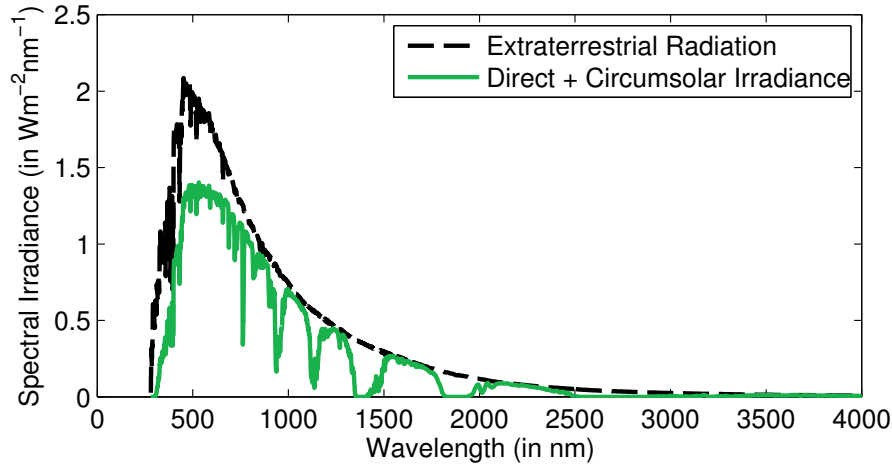
Figure 1.3: Spectral Distribution of Solar Irradiance: The black plot shows the spectral distribution of solar energy above the Earth’s atmosphere. The green plot shows the spectral distribution at the Earth’s surface. There are a few bands of wavelengths in the short wave infrared range which are almost completely absorbed by the atmosphere. Some high end laser range finders operate at these wavelengths but controllable light sources and sensors that work at these wavelengths are not well developed.(Spectral data source: ASTM G-173)
