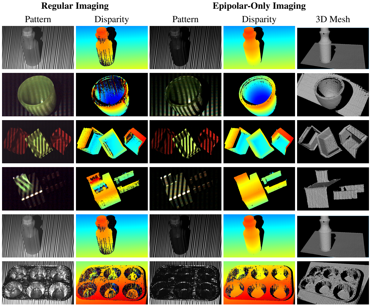
Figure 4.5: Imaging and reconstructing challenging objects with strong global illumination effects. Structured light with regular imaging is prone to errors due to global light transport effects (notice the effects of interreflections on the plastic bins, metal gripper and baking tray. Also observe the subsurface scattering in the green wax bowl). Epipolar-only imaging blocks almost all these effects. Notice how the cross hatching due to interreflections on the gripper has been eliminated and the pattern contrast on the bottle and wax bowl has increased. With the milk bottle, subsurface scattering causes contrast loss and blurring of the projected patterns with regular imaging, with epipolar imaging the patterns appear much sharper and as a result the depth estimates are more accurate. The baking tray is a particularly challenging example. Most of the errors due to specular interreflections have been suppressed, but some regions where interreflections fall along epipolar lines are still reconstructed incorrectly.
