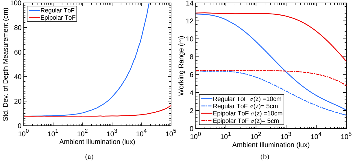
Figure 5.6: A simulation of the standard deviation in depth measurements obtained using regular and epipolar ToF imaging (15 MHz modulation frequency) for a target 10 m from the camera as a function of ambient light level is shown in (a). For both cases, the peak light source power is 2 W and the total exposure time is the same (7.2 ms per image) but epipolar ToF is more robust to ambient light because it concentrates light source power and uses a short exposure for each row (30 \mu\text{s} ). (b) shows the working range of the same simulated camera at different levels of acceptable range accuracy. Note that simulated camera’s parameters differ from prototype, see table 5.2 for parameters and appendix for code listings.
