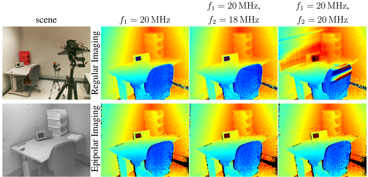
Figure 5.11: Two time-of-flight cameras are placed in a scene. When only one camera is running (second column), both regular imaging and epipolar imaging produce accurate depth maps. With both cameras operate at different frequencies (third column), the depth map with regular imaging becomes noisier because the other camera’s light source adds to the shot noise while epipolar imaging is almost unaffected. When both cameras operate at the same modulation frequency (last column), they interfere strongly in regular imaging mode. With epipolar imaging, the two cameras will usually either not interfere at all, or will interfere along a single line through the image.
