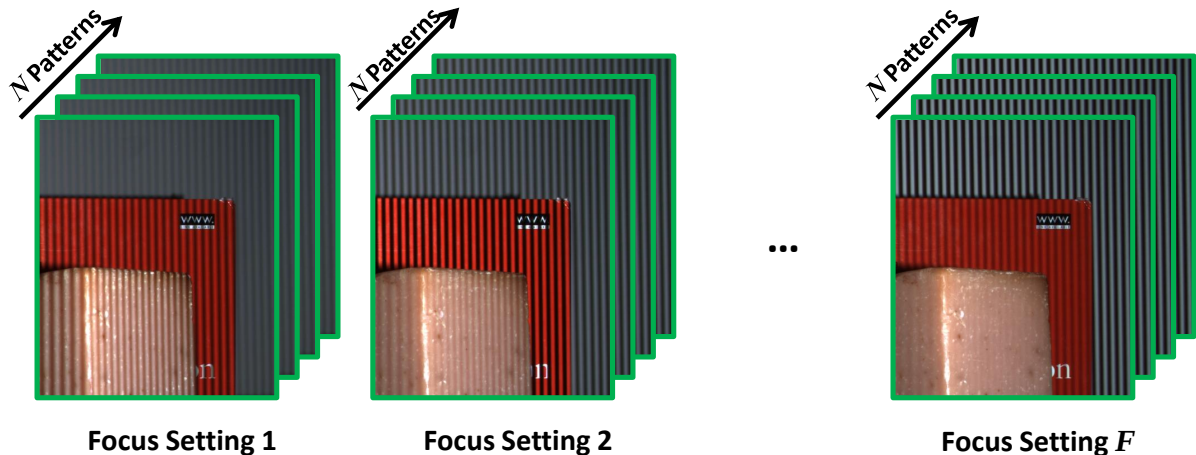
Figure 3.2: Input to our Algorithm: We use binary stripe patterns of varying width. Unlike most other structured light algorithms that use a fixed focus setting on the projector, we change the focus setting to move the plane of focus backwards during the image capture process (the camera focus however remains fixed). We capture a total of T = F \times N images. In our experiments, T typically ranged between 20 and 30. As the figure illustrates, near by objects receive focused illumination in the earlier parts of the sequence and distant objects come into focus later on.
