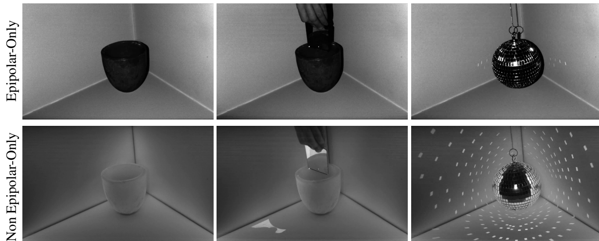
Figure 4.4: Live Transport Probing: Epipolar-only imaging captures direct light transport and the small fraction of global light transport that obeys epipolar geometry. Non Epipolar-only probing captures only global light. These are example frames taken from a video where the sensor alternated between epipolar-only imaging and non epipolar-only imaging. Diffuse interreflections between the walls appear in the non-epipolar image. The wax bowl appears dark in the epipolar-only image because most of its apparent brightness is due to subsurface scattering. Most specular interreflections from the mirror (except those that happen to obey epipolar geometry) appear in the non epipolar-only image.
