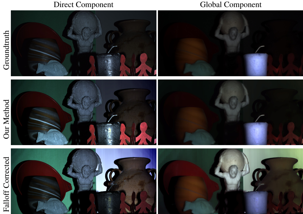
Figure 3.9: Direct-Global Separation. Groundtruth was computed using 112 images and our method used 28. In this scene, the shading on the soap fish and the white statue becomes is very clear in the direct illumination image. As our method also simultaneously recovers depth, we can correct the direct and global images for the the projector fall-off with depth.
