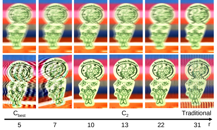
Figure 10. (Left) Visual deblurring comparison of C_2 versus C_{best} on real datasets. Note that the proposed code C_2 gives similar deblurring performance compared to optimal code C_{best} . (Right) PSF estimation capability for n = 31 codes with increasing r (decreasing number of 0 \rightarrow 1 transitions). For small r , PSF estimation fails leading to poor deblurring results. Note that r = 5 for C_{best} , and thus optimal invertible code may not give good PSF estimation. As r increases, PSF estimation improves, but PSF invertibility degrades.
