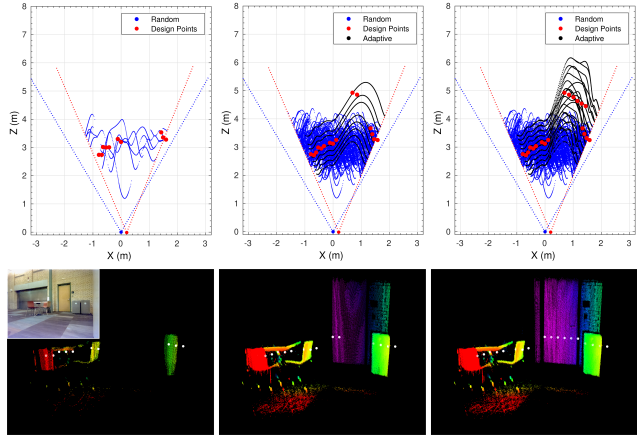
Figure 7: Adaptive depth imaging of a table and chairs scene is performed by first randomly sampling a volume of interest to find objects. Then, the detected points at the front of these objects (indicated by red dots in plots and white dots in bottom row) are used to design a set of light curtains which is then imaged to refine and discover more of the scene. As time continues, the curtains eventually discover and image the back wall of the scene.
