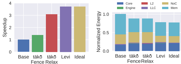
Fig. 5: PHI results for PageRank on a 4M vertex, 40M edge synthetic graph. Leviathan improves performance by 3.7 \times .
