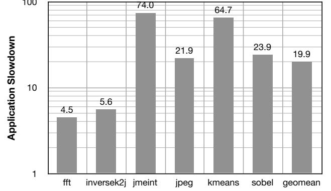
Figure 9: Slowdown with software neural network execution.
