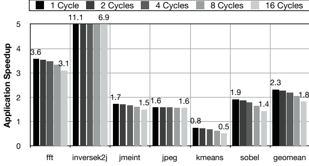
Figure 10: Sensitivity of the application’s speedup to NPU communication latency. Each bar shows the speedup if communicating with the NPU takes n cycles.
