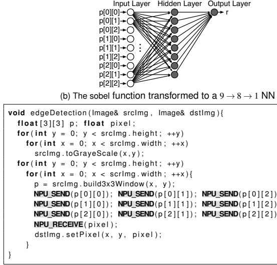
(c) parrot transformed code; an NPU invocation replaces the function call
