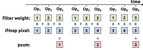
Figure 5. Processing of a 1D convolution primitive in the PE. In this example, R = 3 and H = 5 .
