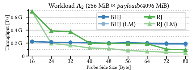
Figure 15: Impact of payload size on join performance
