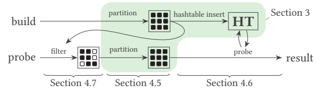
Figure 5: Schematic Overview of our Partitioned Join.
