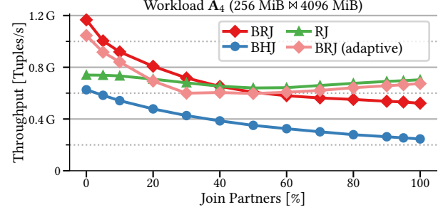
Figure 14: Impact of pre-filtering the probe side using a Bloom-filter based early probe
