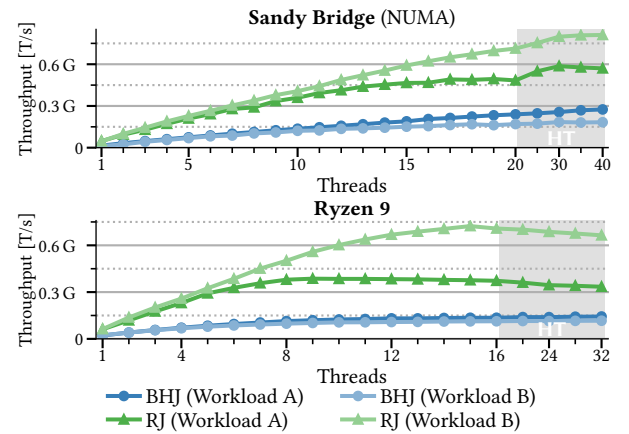
Figure 9: Scalability on different machines
