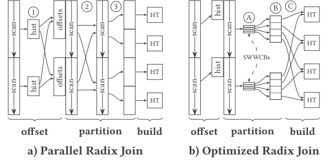
Figure 3: Radix-Partitioning in prior work
