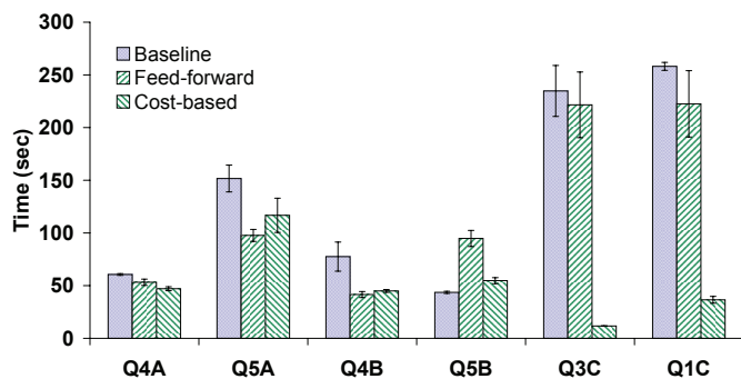
Fig. 13. Running times for join and distributed join queries.
