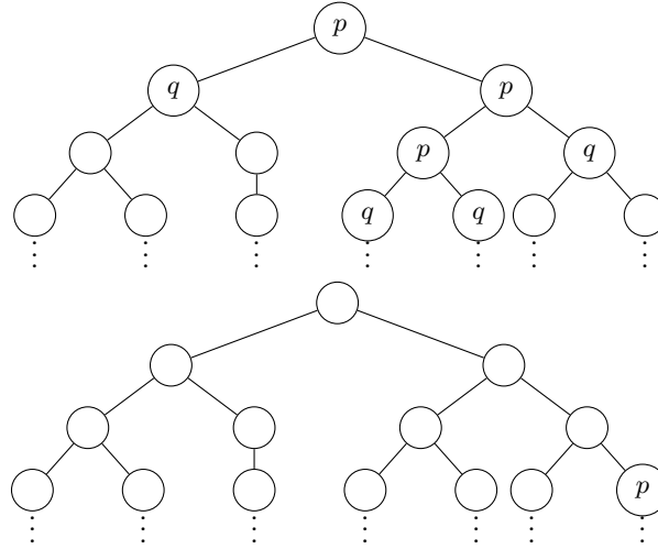
Figure 4: Visualization CTL formulas: A[PUQ] (top) and EFP (bottom).
