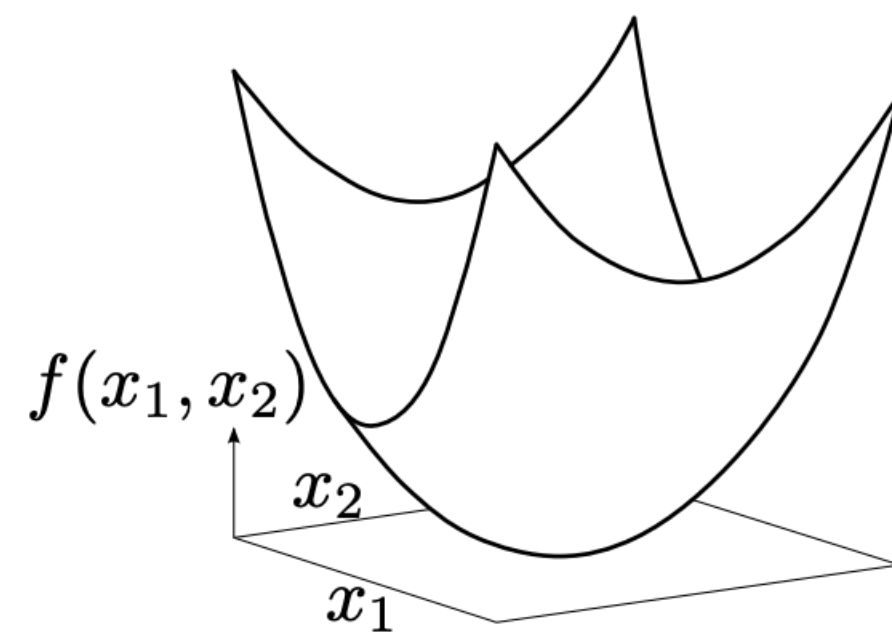
Graph of f(\vec{x})
