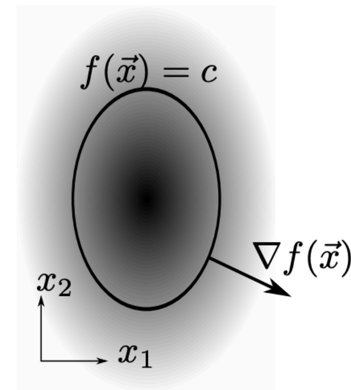
Level sets of f(\vec{x})
