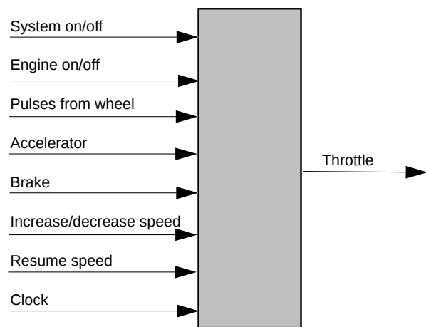
Figure 1.3.1: Block Diagram for Cruise Control.
