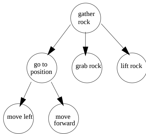
Figure 2.2.7: A Task Tree
