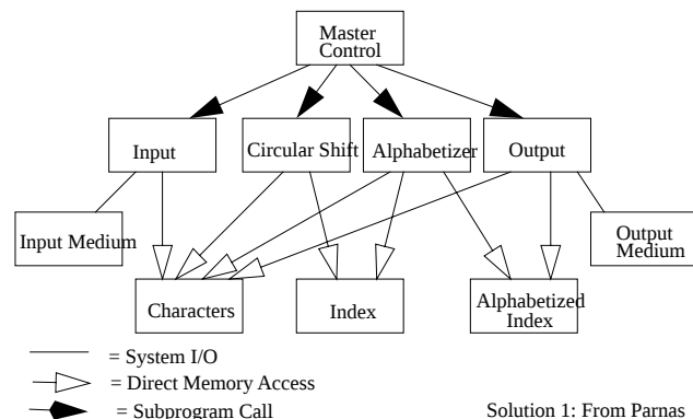
Figure 2.1.2: Hierarchical Subroutine Architecture with Shared Data
