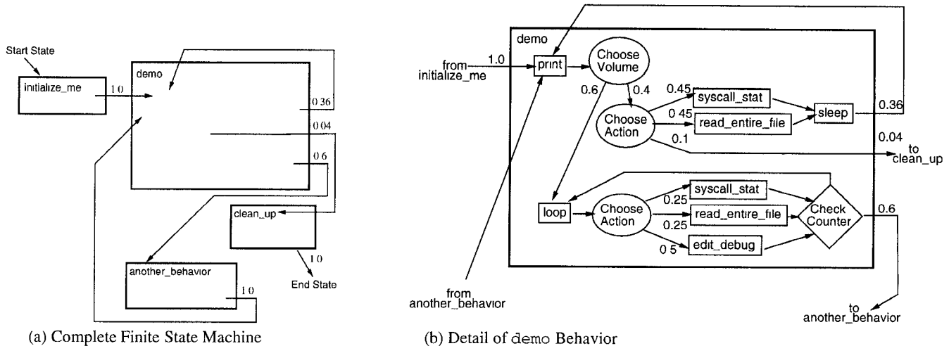
Figure (a) shows the finite state machine for a hypothetical user class. Each of the states initialize_me , demo , clean_up , and another_behavior represent user behaviors. Figure (b) shows the detailed contents of one of these behaviors, demo . Each small rectangle in this figure, such as edit_debug and read_entire_file , corresponds to an action; these actions are implemented in micromodels. In both figures, arcs represent transitions between user behaviors, and the numbers on the arcs indicate transition probabilities.
