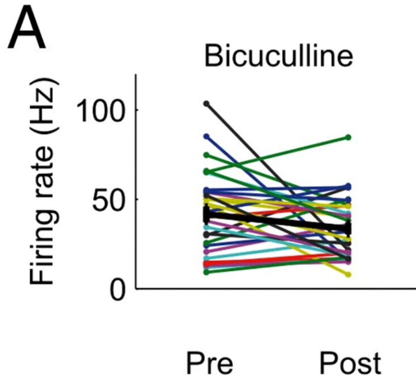
Purkinje cell response to bicuculline
