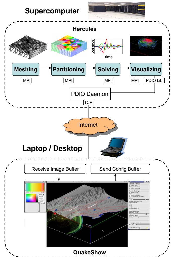
Figure 1: Extended Hercules System Architecture.
