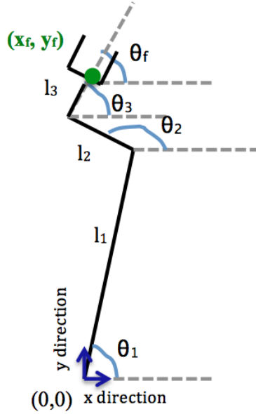
Figure 8: RRR Arm in XY plane with base joint located at (0,0) .
