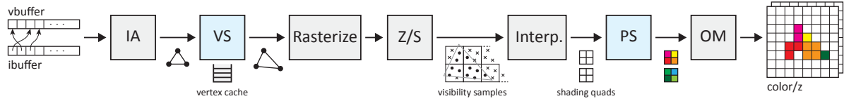
(b) Decoupled Pipeline
