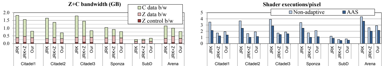
Figure 10: The average bandwidth usage (left) and per pixel shading rate (right) for our test scenes. Our algorithm consumes significantly less bandwidth by keeping the data on chip and achieves nearly the same low shading rate as decoupled sampling with a z -prepass (JRK+Z).
