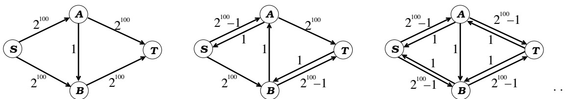
Figure 15.1: A bad case for Ford-Fulkerson. Starting with the graph on the left, we choose the path s - a - b - t , producing the residual graph shown in the middle. We then choose the path s - b - a - t , producing the residual graph on the right, and so on.
