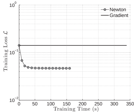
Fig. 2. Gradient vs. Newton steps in alternating projection.
