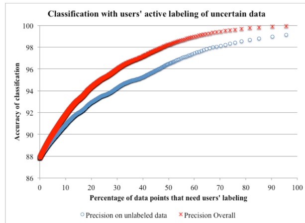
Figure 3. Classification with uncertainty
