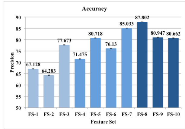
Figure 2. Accuracy of Predictions
