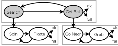
Fig. 1. An example soccer-related skill hierarchy. The robot will search for the ball, and then run up and grab it. Transitions are conditioned on the robot’s perceptual beliefs.
