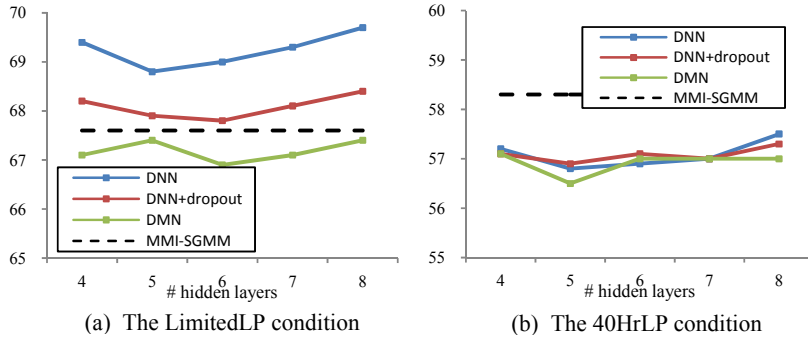
Fig. 2. WERs(%) for MMI-SGMM and hybrid systems on the dev set. DNN and DNN+dropout are pre-trained with SDAs while DMN is randomly initialized.
