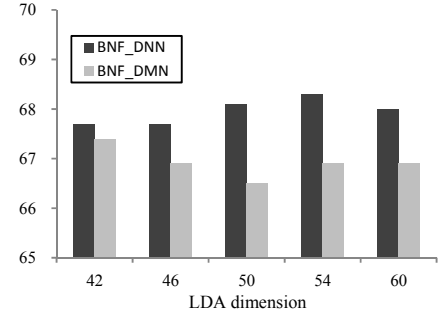
Fig. 3. WERs(%) for LimitedLP BNF systems on the dev set. Comparison is made between DNNs and DMNs.
