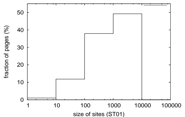
Figure 3: Histogram of distribution over number of pages hosted by sites of different size. The x -axis gives the magnitude of the number of pages hosted by a site, and the y -axis shows the fraction of pages hosted by all sites of that size.
