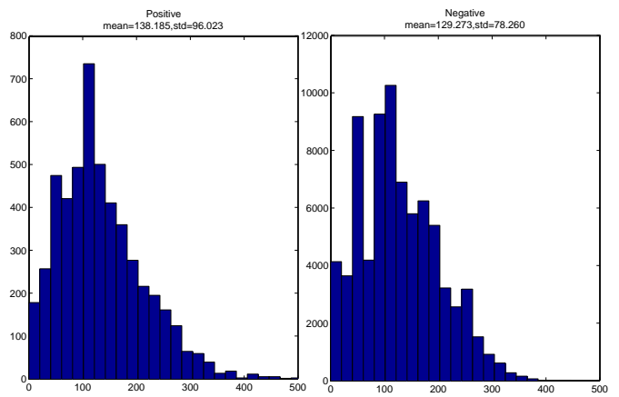
Figure 1: The histograms of proximity feature values from positive examples (left) and negative examples (right)
