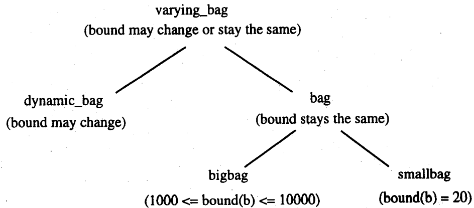
Figure 3 A Type Family for Bags
