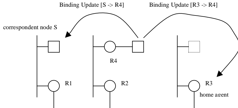
Figure 3. Binding Update messages
