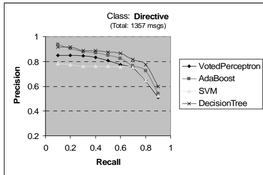
Figure 4 - Precision/Recall for Directive act
