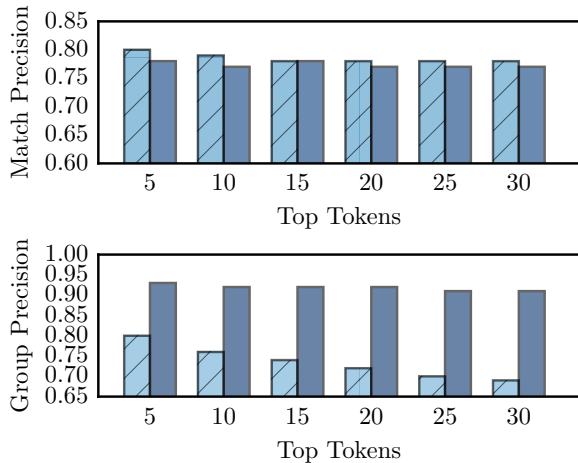
Figure 2: Average Match (top) and Group (bottom) precision of top tokens of 50 topics learned with KB-LDA, according to expert (dark blue) and non-expert (light blue, stripes) labeling.
