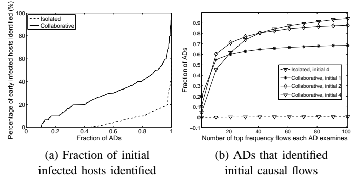
Fig. 9. The ability to identify the initial infected hosts and the attack entry point with and without collaboration for each AD.
