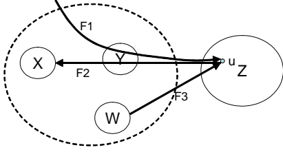
Fig. 4. An example partial deployment scenario. W , X , Y are three ADs that are in the federation, and AD Z does not participate. F1 , F2 , and F3 represent three network flows to or from host u in AD Z .
