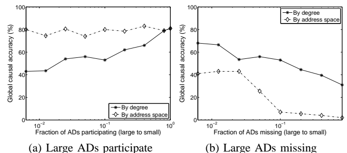
Fig. 10. Global detection accuracy under different missing scenarios, with the random scanning worm. We use the best recovery strategy, i.e., routing horizon -based recovery.
