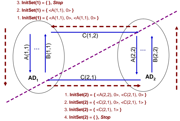
Fig. 3. A simple example with two domains collaborating in the distributed protocol. Solid arrows represent the direction of network flows, and dashed arrows represent the direction of random moonwalks (reversed with respect to the flow directionality).
