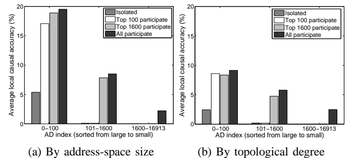
Fig. 13. Benefits of participation under partial deployment, assuming the large ADs participate
