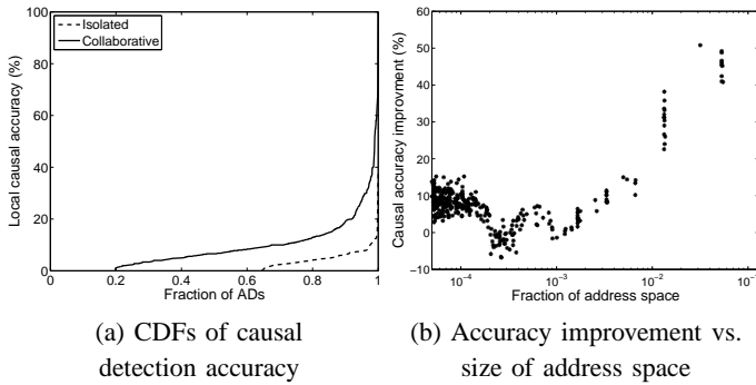
Fig. 8. Causal flow detection accuracy with and without collaboration for each AS ( Z = 100 ).
