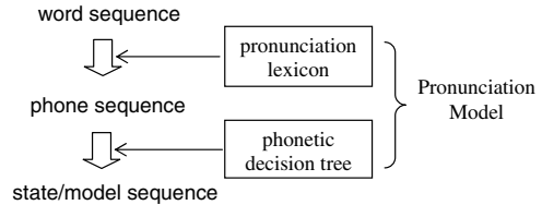
Figure 1: Pronunciation model as a mapping from symbolic level to model level
