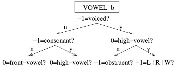
Figure 4: Top part of Vowel-b tree (beginning state of vowels). “-l=” questions ask about the immediately left phone, “0=” questions ask about the center phone.
