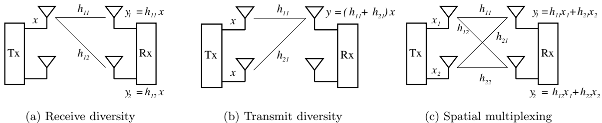
Figure 2: Using some of the transmit/receive antennas in an example 2x2 system to exploit diversity and multiplexing gain. x_i and y_i represent transmitted and received signals. The channel gain h_{ij} is a complex number indicating a signal's attenuated amplitude and phase shift over the channel between the i th transmit antenna and the j th receive antenna. The received signals y_i will additionally include thermal RF noise.
