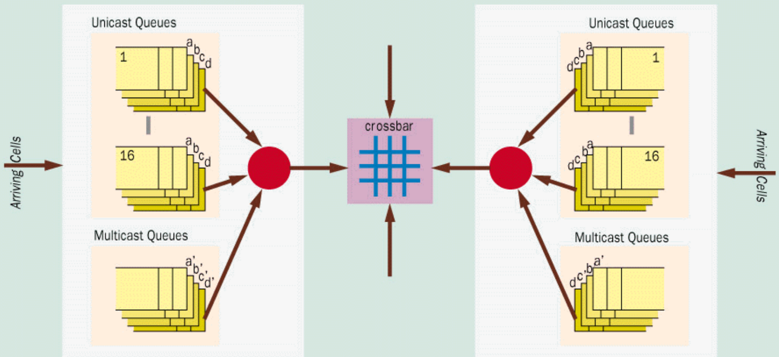
FIGURE 11 Queues Maintained for a 16-port Unicast-Multicast Switch
