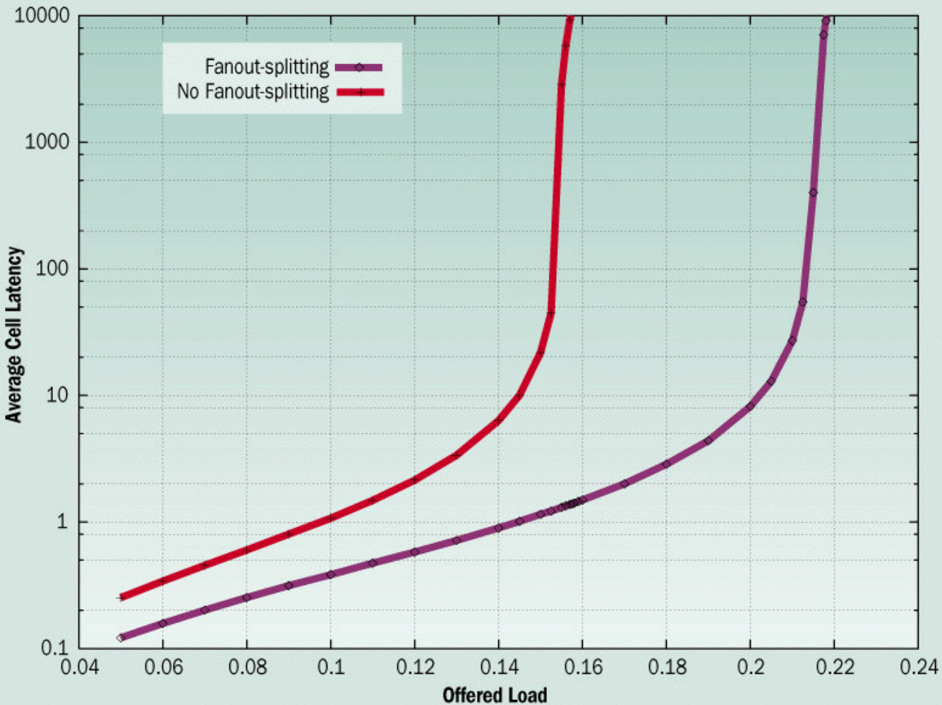
FIGURE 10 Average Cell Latency with and without Fanout Splitting
