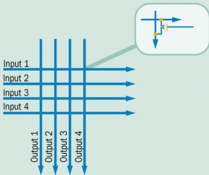
FIGURE 4 A Four-Input Crossbar Interconnection Fabric
