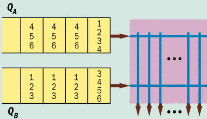
FIGURE 9 A 2 \times N Crossbar Switch that Supports Multicast
