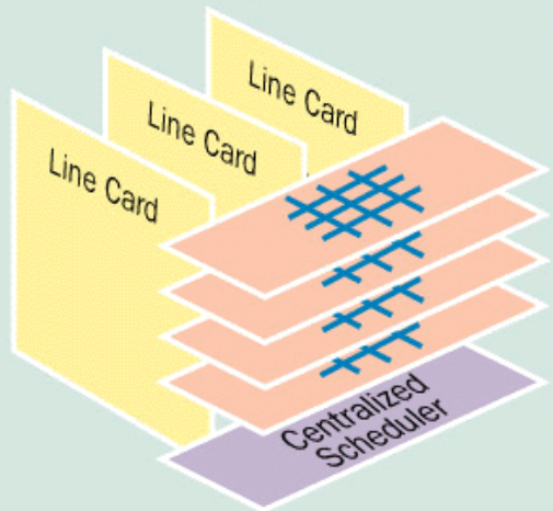
FIGURE 5 A Four-Way Parallel Crossbar Switch, Interconnecting Three Line Cards
