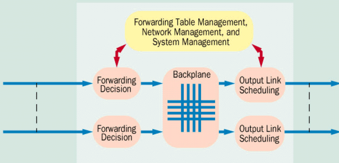
FIGURE 1 The Key Common Architectural Components of a Router
