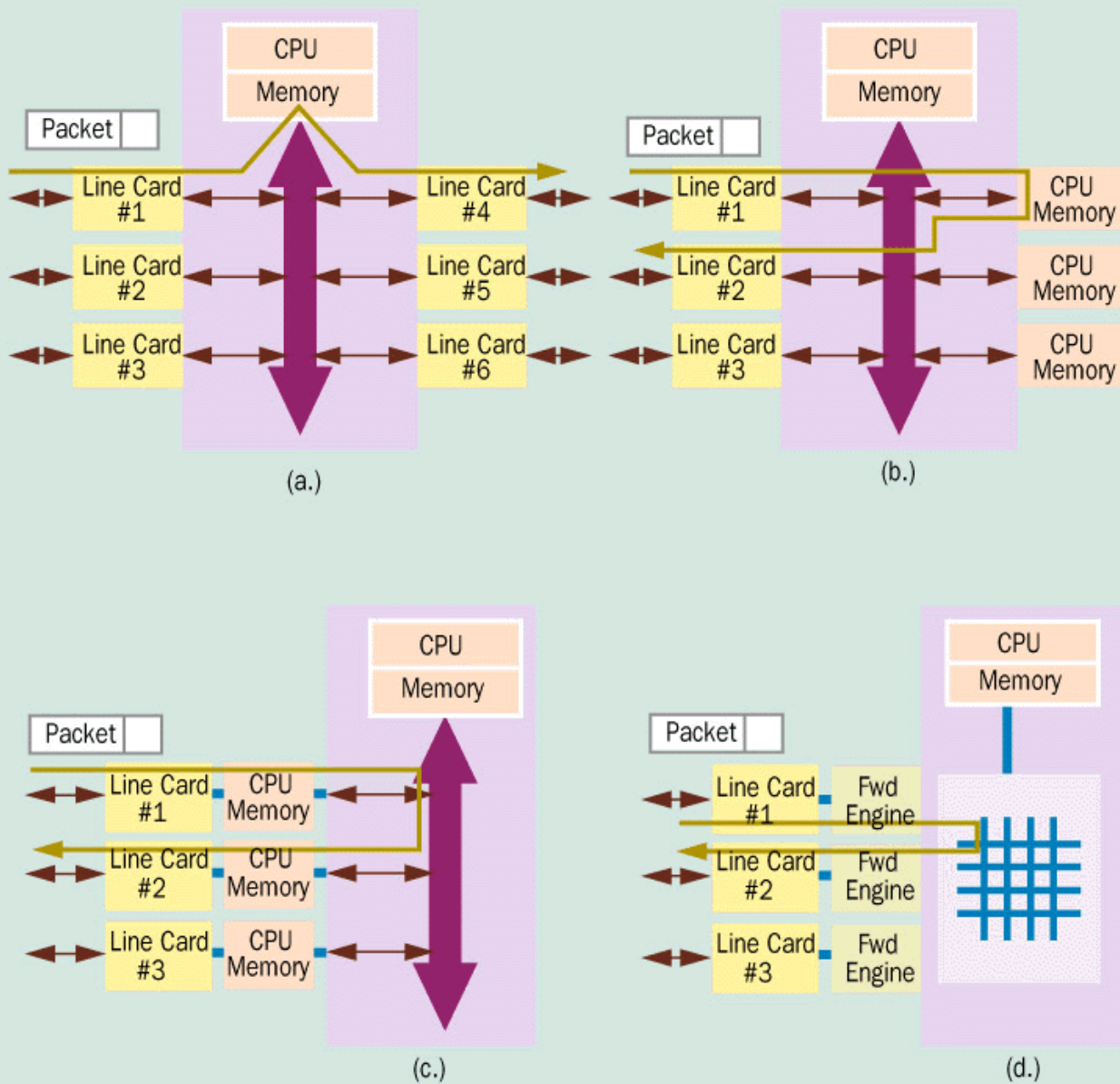
FIGURE 2 The Basic Architectures of Packet Processors
