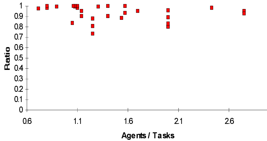
Simulation task execution / Optimal task execution
