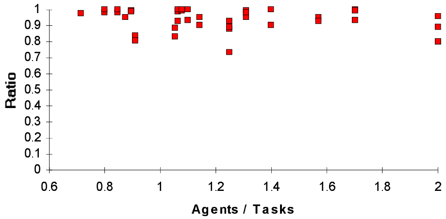
Simulation task execution / Optimal task execution
