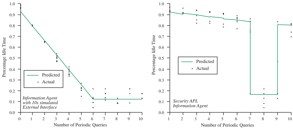
Figure 3: On the left, graph of predicted and actual utilization for a real information agent with a simulated external query interface. On the right, the same graph for the Security APL stock ticker agent.
