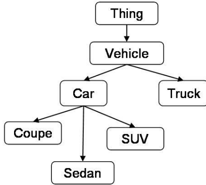
Figure 4. Vehicle Ontology
