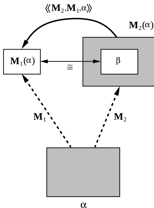
Figure 7.3 When one model contains another, a unique pairing connects the graphs they produce. Here we see that \mathbf{M}_1 \subseteq \mathbf{M}_2 , so \mathbf{M}_1(\alpha) is isomorphic to a subgraph \beta of \mathbf{M}_2(\alpha) . The containment map \langle\langle \mathbf{M}_2, \mathbf{M}_1, \alpha \rangle\rangle acts on all of \mathbf{M}_2(\alpha) to take this subgraph \beta back to \mathbf{M}_1(\alpha) .
