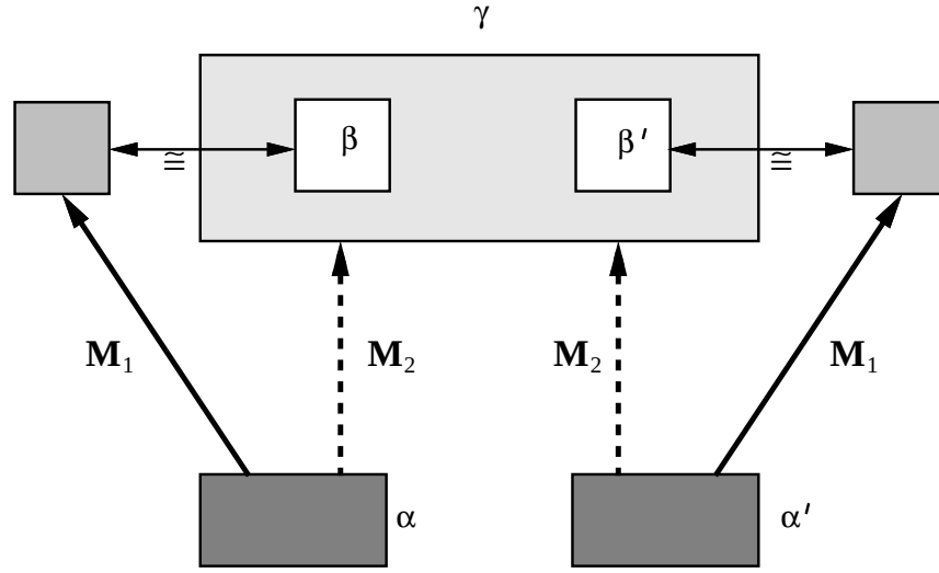
Figure 7.5 Containment does not guarantee well-defined components. Although M_1 \widetilde{\subseteq} M_2 model M_1 may be isomorphic to different subgraphs depending on the original graph. Here, \gamma = M_2(\alpha) = M_2(\alpha') but \beta , the subgraph isomorphic to M_1(\alpha) differs from \beta' , the subgraph isomorphic to M_1(\alpha') .
