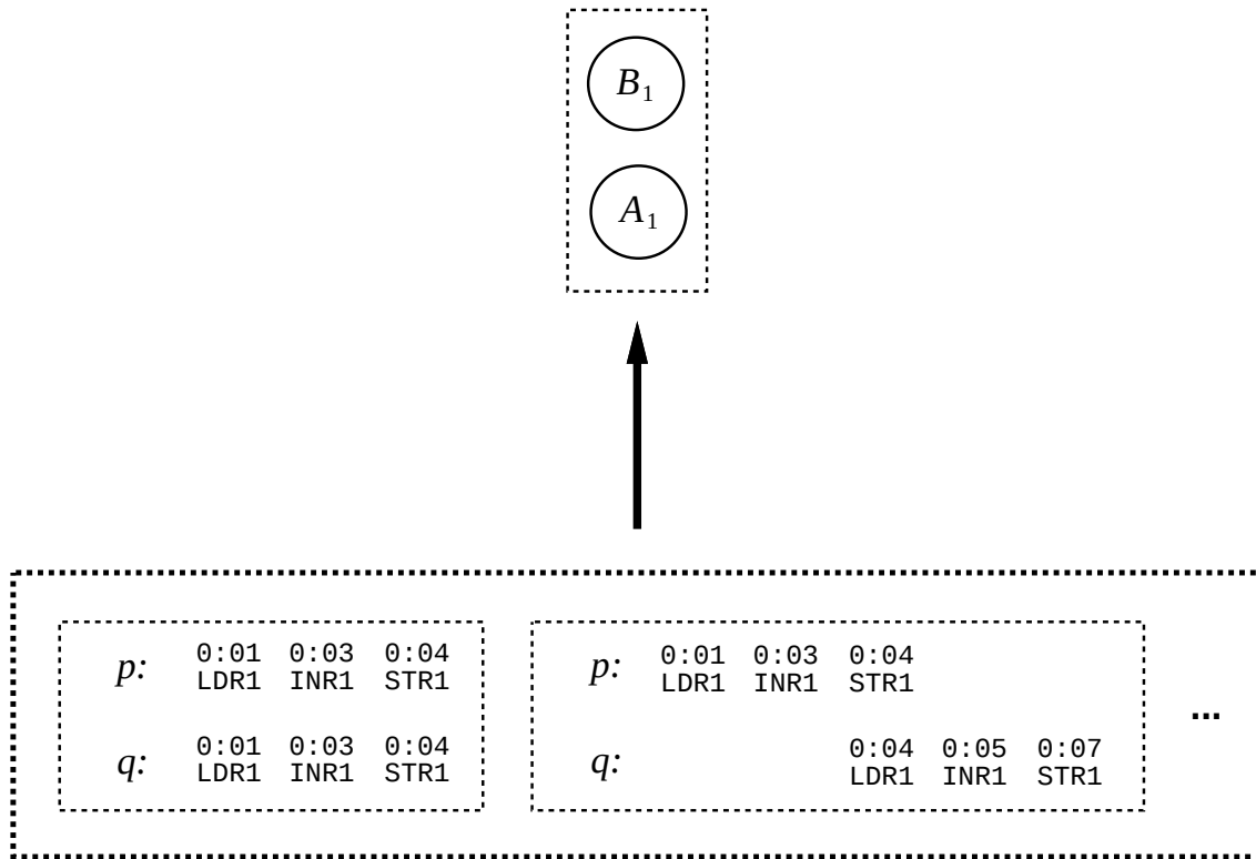
Figure 1.6 An abstract computation graph represents a set of possible physical computations. Once we abstract to the graph, we forget the presumably irrelevant physical detail.
