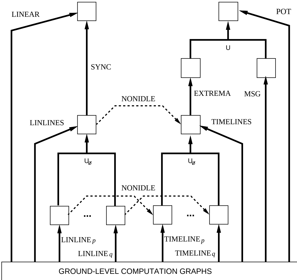
Figure 6.1 The models we discuss here fit into a composition hierarchy. The boxes indicate sets of computation graphs; an arrow \mathbf{M} between two boxes indicates that model \mathbf{M} is a surjection from the one set onto the other. What's more, the functional identities we illustrate here are also model identities—e.g., the model \mathbf{LINEAR} equals the composition of models \mathbf{SYNC} \circ \mathbf{LINLINES} .
