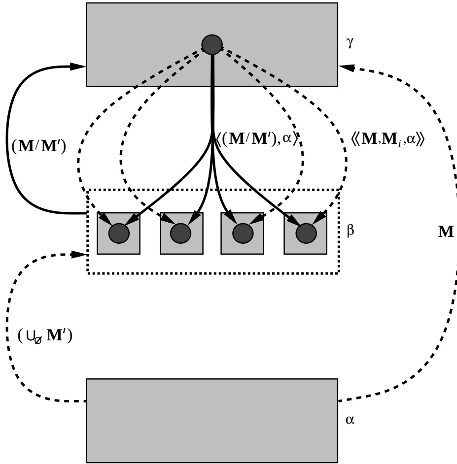
Figure 7.7 Model \mathbf{M} with decomposition \mathbf{M}' induces a factoring model \mathbf{M}/\mathbf{M}' . The decomposition \mathbf{M}' = \cup_{\emptyset} \{\mathbf{M}_i\} takes \alpha (bottom) to \beta (middle); the model \mathbf{M} takes \alpha to \gamma (top). The factoring model \mathbf{M}/\mathbf{M}' takes \beta to \gamma ; in the new model, an atom of \gamma represents the union of its images in each \mathbf{M}_i component. (Solid arrows indicate both the action and the representation of the new model. Dashed arrows indicate the action of \mathbf{M} , \mathbf{M}' , and the containment maps.)
