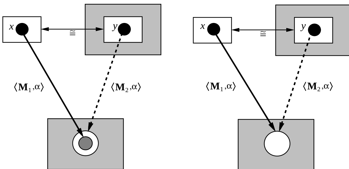
Figure 7.2 If M_1 \widetilde{\subseteq} M_2 , then the M_1 representation on any atom x yields a subset of what the M_2 representation yields on the matching atom y (left). For strong containment M_1 \overline{\subseteq} M_2 , the representations are equal (right).
