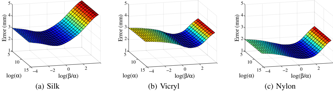
Fig. 3: Static error landscapes for isotropic DOOs. We use Equation (2) as the error and show the error landscapes for silk, vicryl, and nylon DOOs. The parameters with lowest test error are different for each type of DOO.
