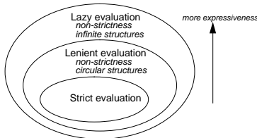
Figure 2: Expressiveness of the three evaluation strategies.
