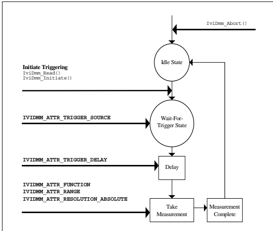
Figure 4-1. IviDmm Behavior Model
