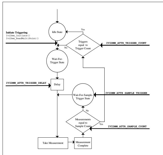
Figure 11-1. IviDmmMultiPoint Behavior Model
