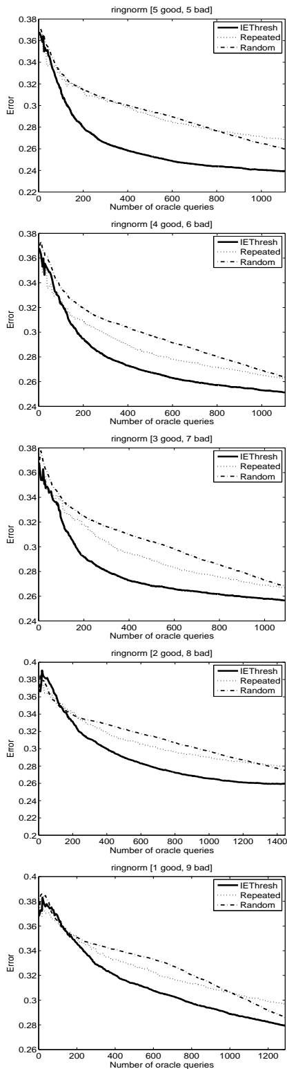
Figure 3: Average classification error vs. total number of oracle queries on ringnorm dataset. For the top figure, accuracy \in [.8, 1] for k_{good} = 5 labelers and accuracy \in [.5, .7] for the remaining k_{bad} = 5 labelers. k_{good} decreases down to 1 and k_{bad} increases up to 9 from top to bottom.
