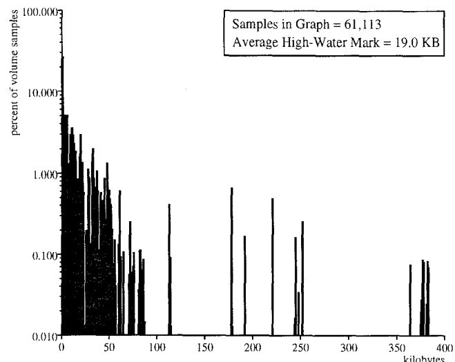
This graph shows the distribution of the maximum resolution log size reached each day by each volume. The high-water mark is reset each morning to the current log size. Note that the y axis is log 10 scaled.
