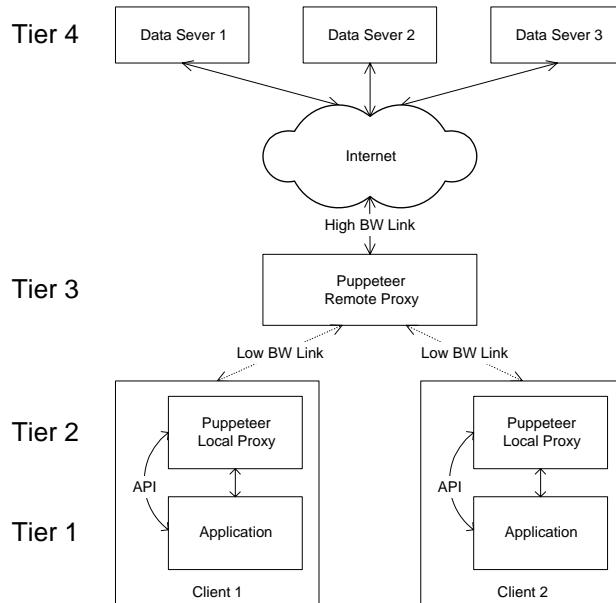
Fig. 1. Puppeteer architecture
