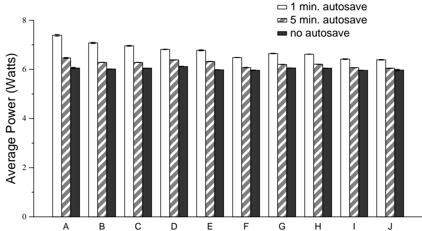
This figure shows how the frequency of PowerPoint autosave affects power usage. The three bars in each data set show power use with a 1 minute autosave frequency, with a 5 minute autosave frequency, and with autosave disabled. Each bar represents the mean of five trials—the error bars show 90% confidence intervals.
