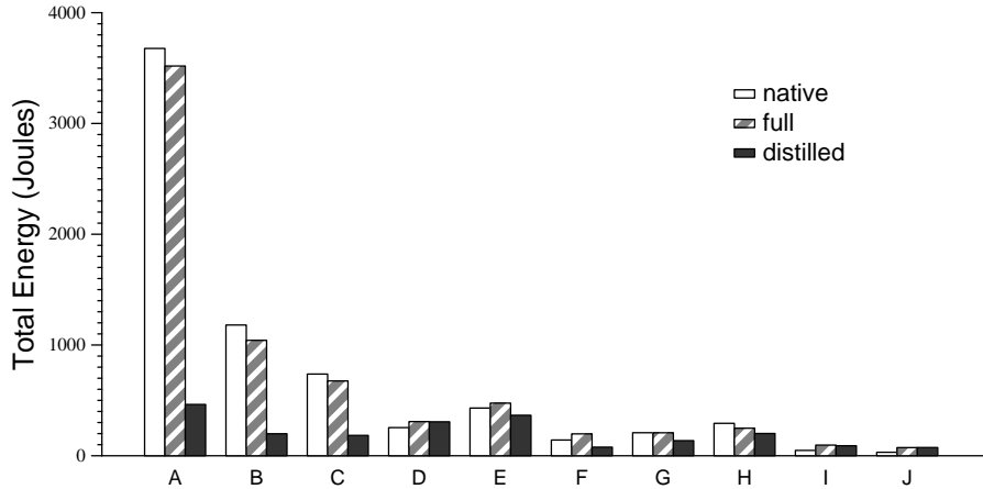
This figure shows the energy used to load ten PowerPoint presentations from a remote server. Native mode loads presentations from an Apache Web server. Full and distilled modes load presentations from a remote Puppeteer proxy, with full mode loading the entire presentation and distilled mode loading a lower-quality version. On average, distilled mode uses 60% of the energy of native mode. Each bar represents the mean of five trials—90% confidence intervals are sufficiently small so that they would not be visible on the graph.
