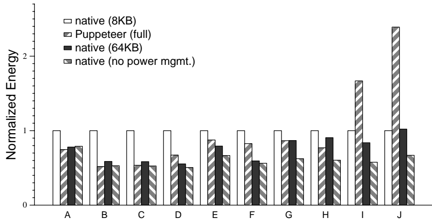
This figure shows how network parameters influence the energy needed to load applications from a remote server. The scenarios used to generate the bars in each data set are identical to those described in Figure 10. Each bar represents the mean of five trials—90% confidence intervals are sufficiently small that they would not be visible on the graph.
