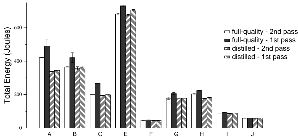
This figure shows the amount of energy needed to page through a presentation a second time. The energy needed to page through each presentation the first time is also shown for comparison. For each data set, the left two bars show energy use for a full-quality presentation loaded using native mode, and the right two bars show energy use for a reduced-quality version. Each bar represents the mean of five trials—the error bars show 90% confidence intervals.
