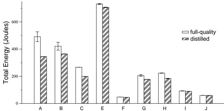
This figure shows the amount of energy needed to page through a presentation. For each data set, the left bar shows energy use when a full-quality presentation is loaded using native mode, and the right bar shows energy use for a reduced-quality version of the same presentation. Each bar represents the mean of five trials—the error bars show 90% confidence intervals.
