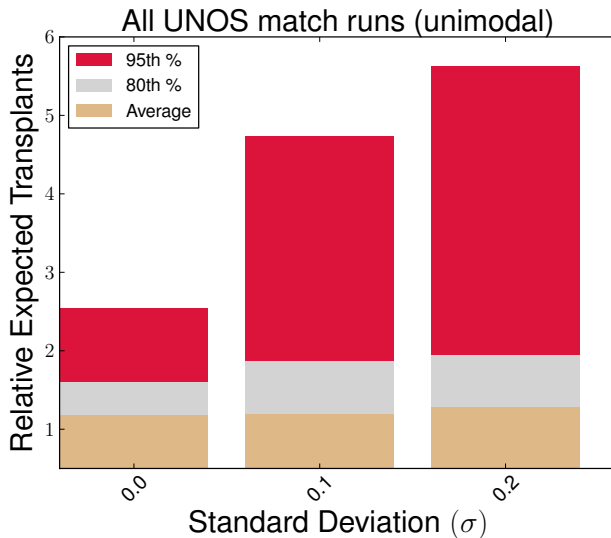
Figure 5 Aggregate additional transplants over all UNOS match runs through November 2013, for edge failure probabilities drawn randomly from \mathcal{N}(\mu = 0.7, \sigma \in \{0.1, 0.2\}) . The leftmost point “ \sigma = 0.0 ” represents a constant failure rate of 70%.
