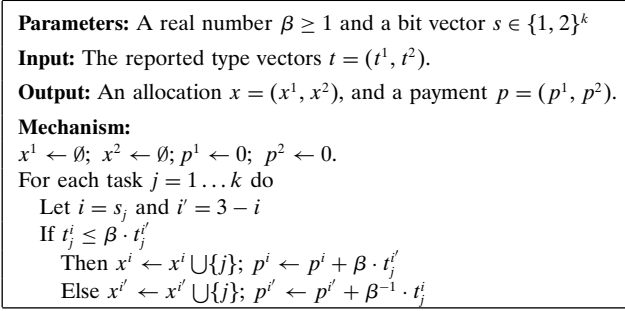
FIG. 1. The biased min work mechanism (for two agents).
