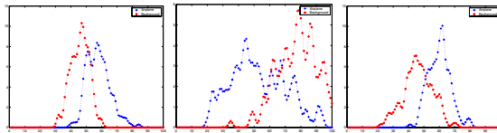
Figure 5: Histograms of three different feature dimensions used in training of Airplane-Background Classification. Blue and Red represent airplane and background respectively.
