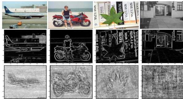
Figure 3: In top to bottom form, each image is followed by its gradient and reconstructed image structure from top 150 eigenvectors. Categories are Airplane, Motorcycle, Leafs and Background. Note how well the top eigenvectors cover the main structure while remaining components pick up the noise. No consistent structure present in the background is reflected in its reconstruction.
