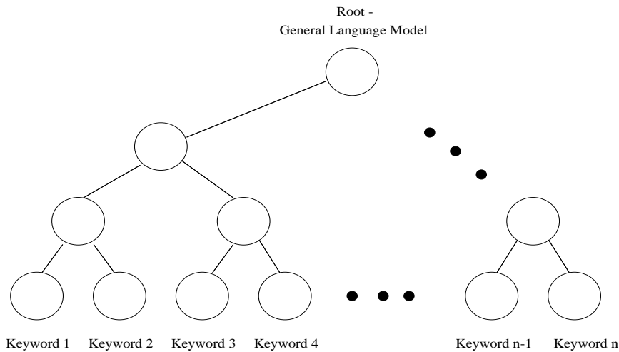
Figure 2: A topic tree built from keyword clusters.
