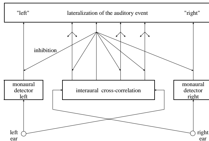
Figure 2-5. Conceptual Representation of Lindemann model. The interaural crosscorrelation model is extend with monaural detectors and inhibition mechanisms.
