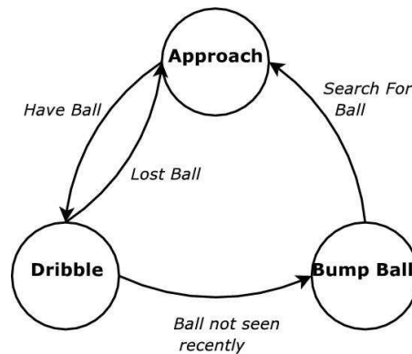
Fig. 7. Finite state machine for the dribble behavior.
