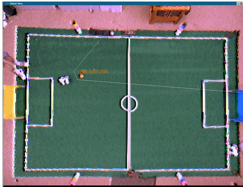
Fig. 11. Overhead camera view with world state information superimposed on it. This image shows the robot's position with uncertainty, the field of view of the camera, and an estimate of the ball's position in the image.
