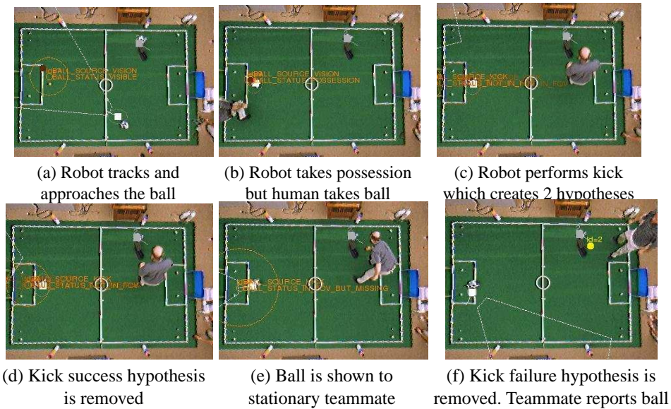
Fig. 6. An illustrative example of the multi-hypothesis algorithm. These images show a top-down view of the soccer field superimposed with world model log information captured live from the robots. This demonstrates how the multiple hypothesis estimation algorithm directs the robot's actions. The robot attempts to kick the ball but the ball is moved by an anonymous human before the kick is completed. The robot tracks cycles through the available hypotheses before switching to listen to its teammate. The straight dashed lines show the robot's expected field of view of the field.
