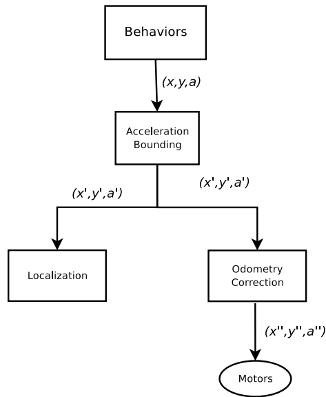
Fig. 8. Overview of the odometry pipeline.
