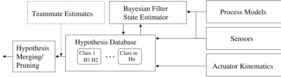
Fig. 5. Dataflow diagram for the multiple hypothesis space state estimator. Environment information from sensors, kinematic models of the robot’s actuators and sensor poses, and a library of sensor models are used to support a database of probabilistic hypothesis about the state of the world. Different hypotheses can belong to different classes, depending on the source of information which created them. Each hypothesis is updated by a Bayesian filter and a post-processing decision process uses domain knowledge to merge relevant estimates and prune those that are of lesser value. Teammate information is also considered, but only at the post-processing phase.
