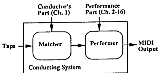
Figure 1: The conducting system consists of a Matcher that associates incoming beats with the conductor's part, and a Performer that schedules output messages.
