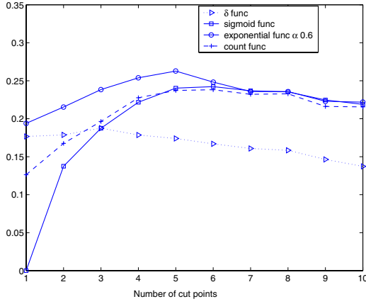
Figure 3. Averaged F_1 measure for the Coref dataset
